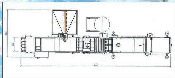
BATTER AND BREAD COATING LINE
